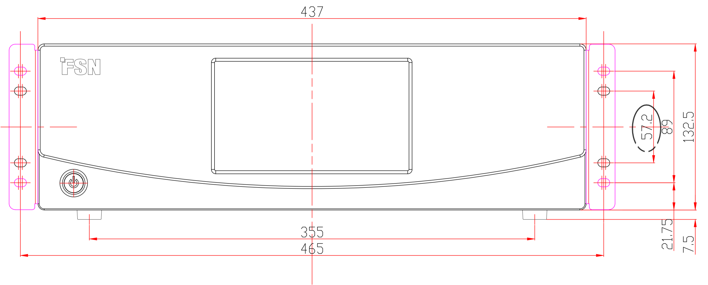
AFTER IPS4000 Assemble (With Rack Mount BRKT)
